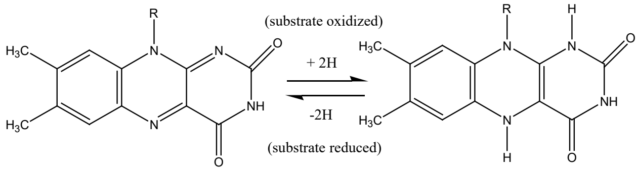
FAD
